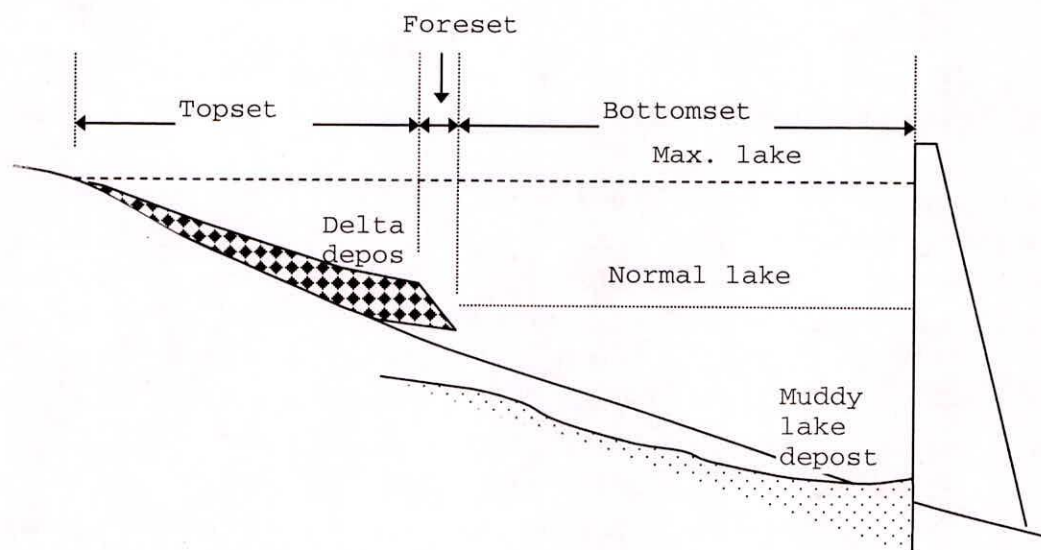
Fig. 1 Sediment deposit zones in a reservoir.
