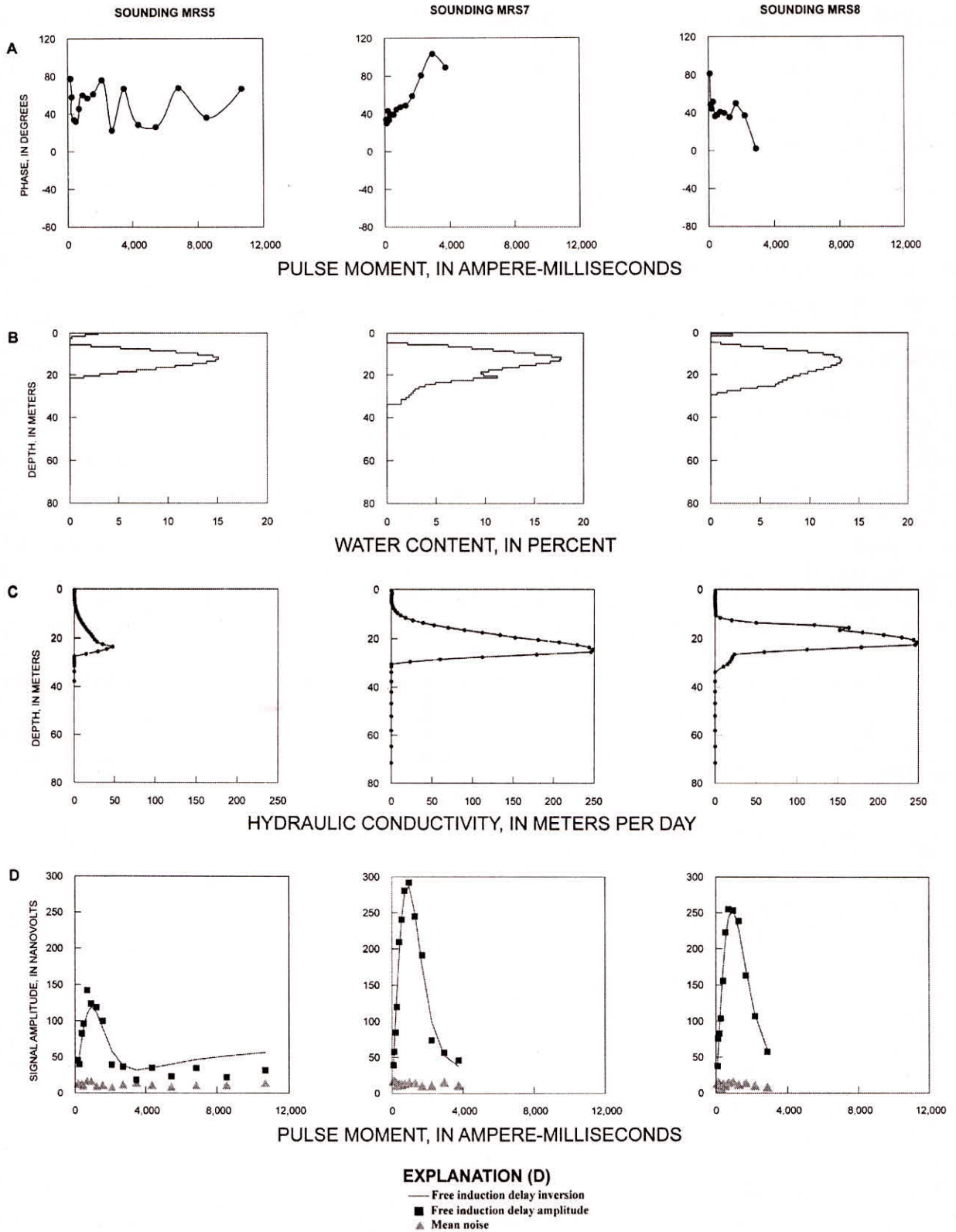
Fig. 4: Magnetic Resonance Sounding (MRS) inversion results: (A) phase relative to pulse moment, (B) depth relative to water content, (C) depth relative to hydraulic conductivity, and (D) pulse moment relative to signal amplitude with signal-to-noise indication
