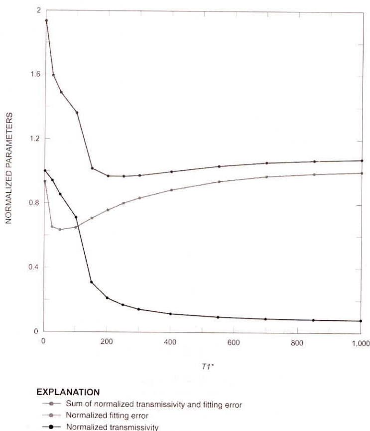
Fig. 5: Calibration graph used to obtain the optimum relaxation time ( T1^* ) for inversion of magnetic resonance sounding data using the default coefficient of permeability ( Cp ) value of 7.00 \times 10^{-9} , Brazos River Hydrologic Field Research Site, College Station, Texas
