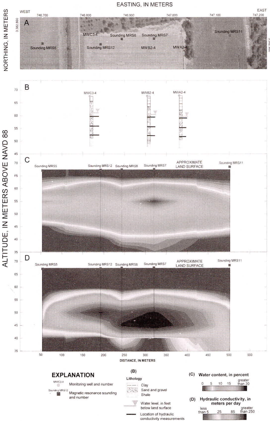
Fig. 7: (A) Location of selected wells and Magnetic Resonance Soundings (MRS), (B) drillers' logs with static water-level and locations of hydraulic conductivity measurements, (C) gridded percentage water content profile, and (D) gridded hydraulic conductivity profile based on MRS results, Brazos River Hydrologic Field Research Site, College Station, Texas
