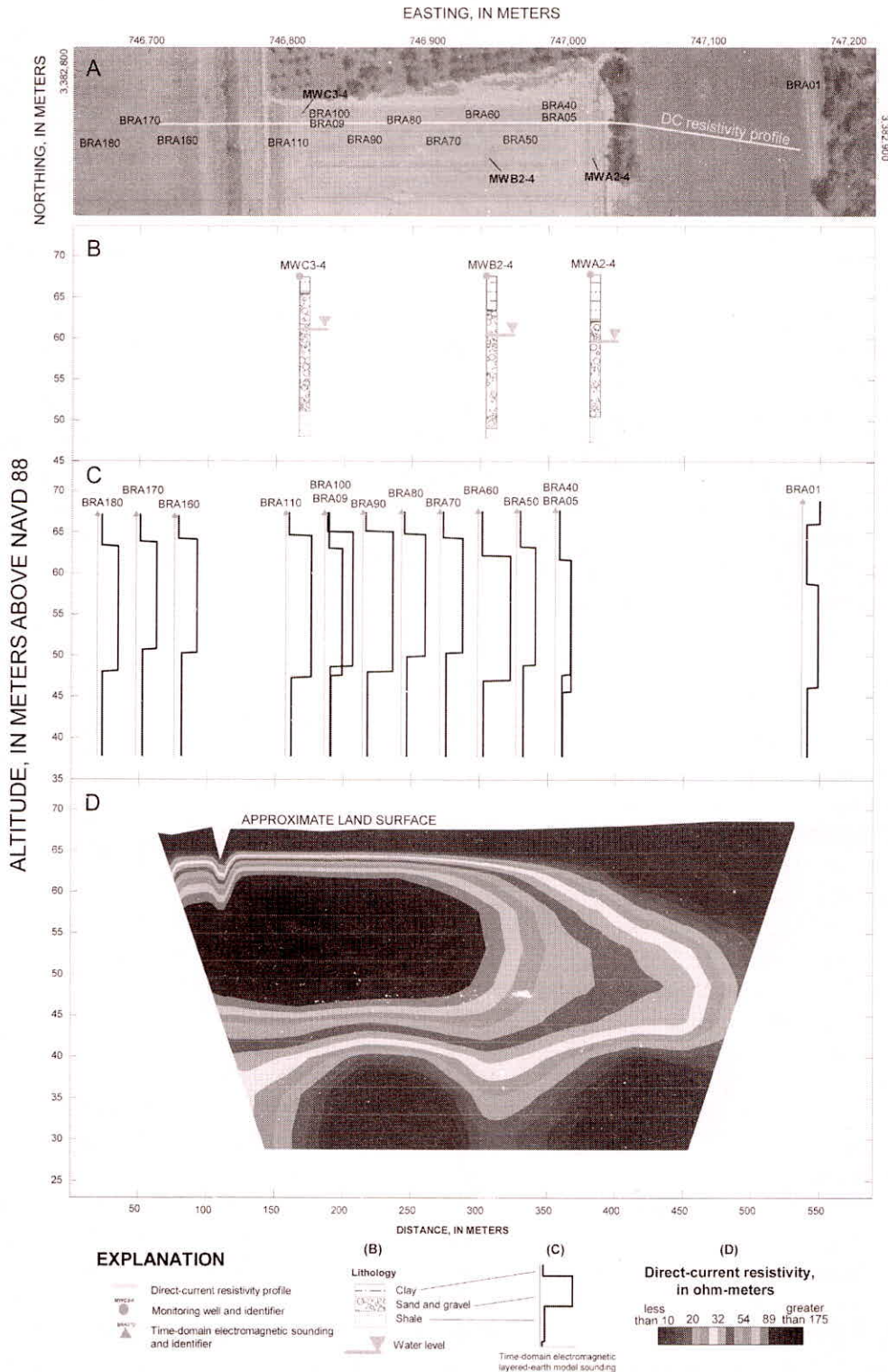
Fig. 6: (A) Location of selected wells and time-domain electromagnetic (TDEM) soundings, (B) drillers' logs with static water level, (C) TDEM layered-earth model sounding results, and (D) robust inversion profile of two-dimensional direct-current dipole-dipole resistivity array, Brazos River Hydrologic Field Research Site, College Station, Texas
