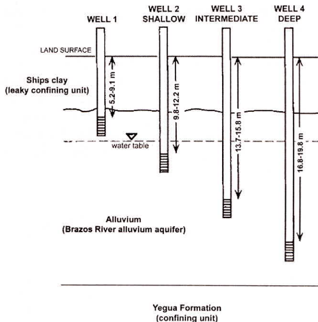
Fig. 3: Schematic of well nest layout, Brazos River Hydrologic Field Research Site, College Station, Texas
