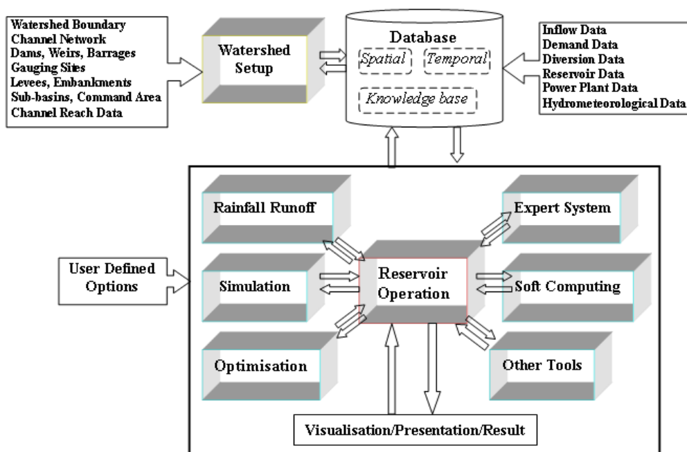
Fig. 3 : Proposed Structure of DSS for Reservoir Management
