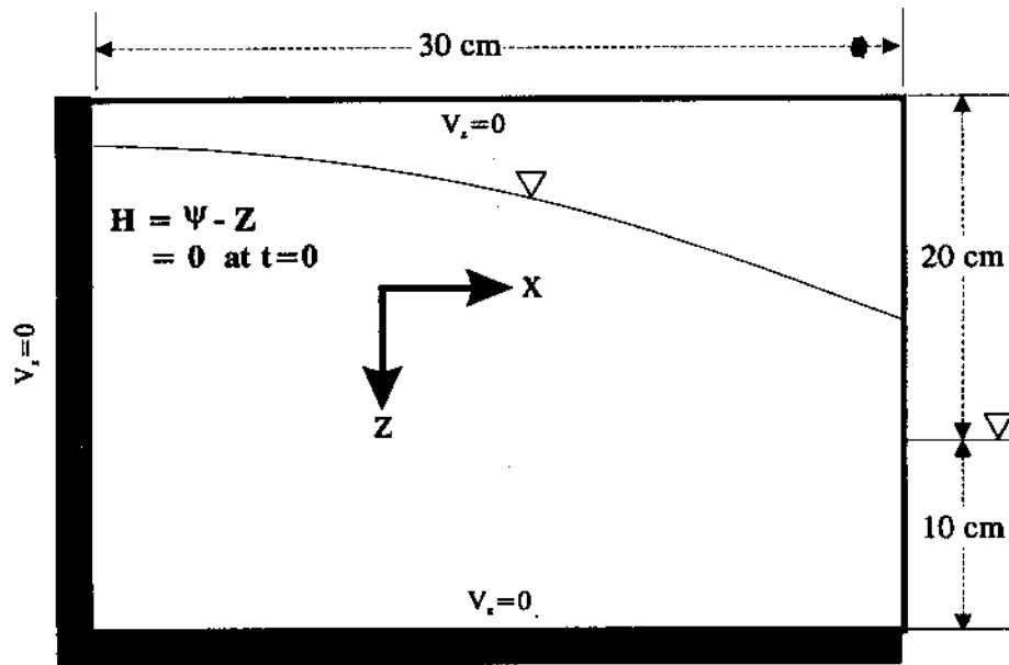
Fig. 3 Problem Definition Sketch for validation
