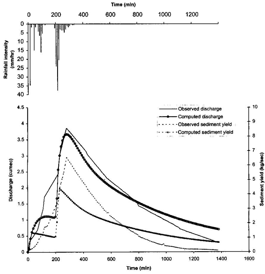
Fig. 9 Comparison of observed and simulated discharge and sediment yield (04.08.1991)
