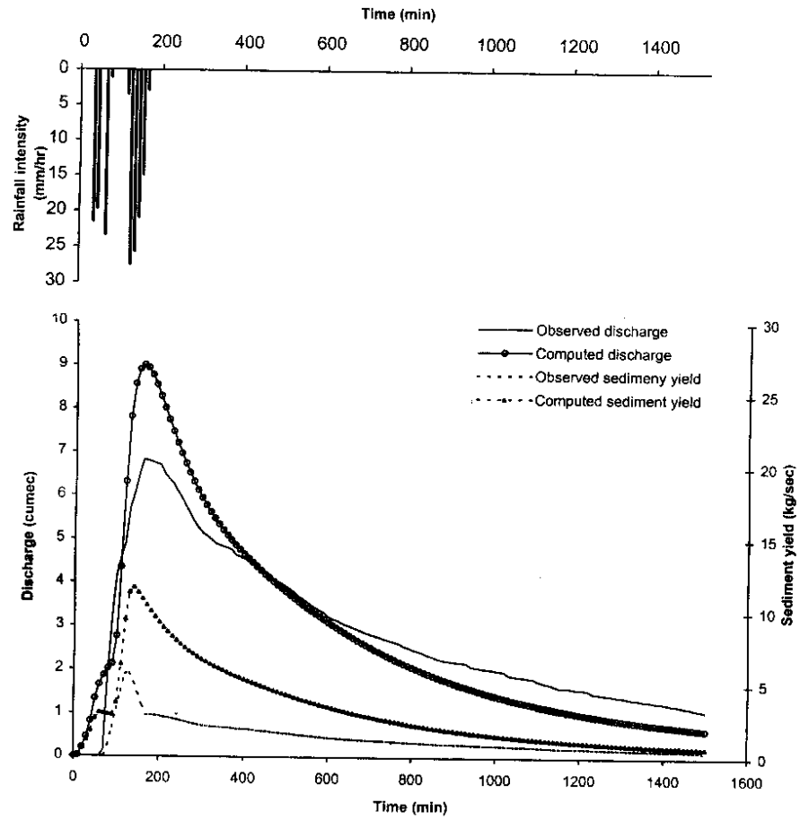
Fig. 11 Comparison of observed and simulated discharge and sediment yield (27.07.1991)
