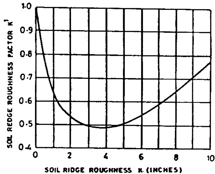
Fig.4 Chart to determine soil ridge roughness factor K' from the soil ridge roughness K_r (Woodruff and Siddoway, 1965)
