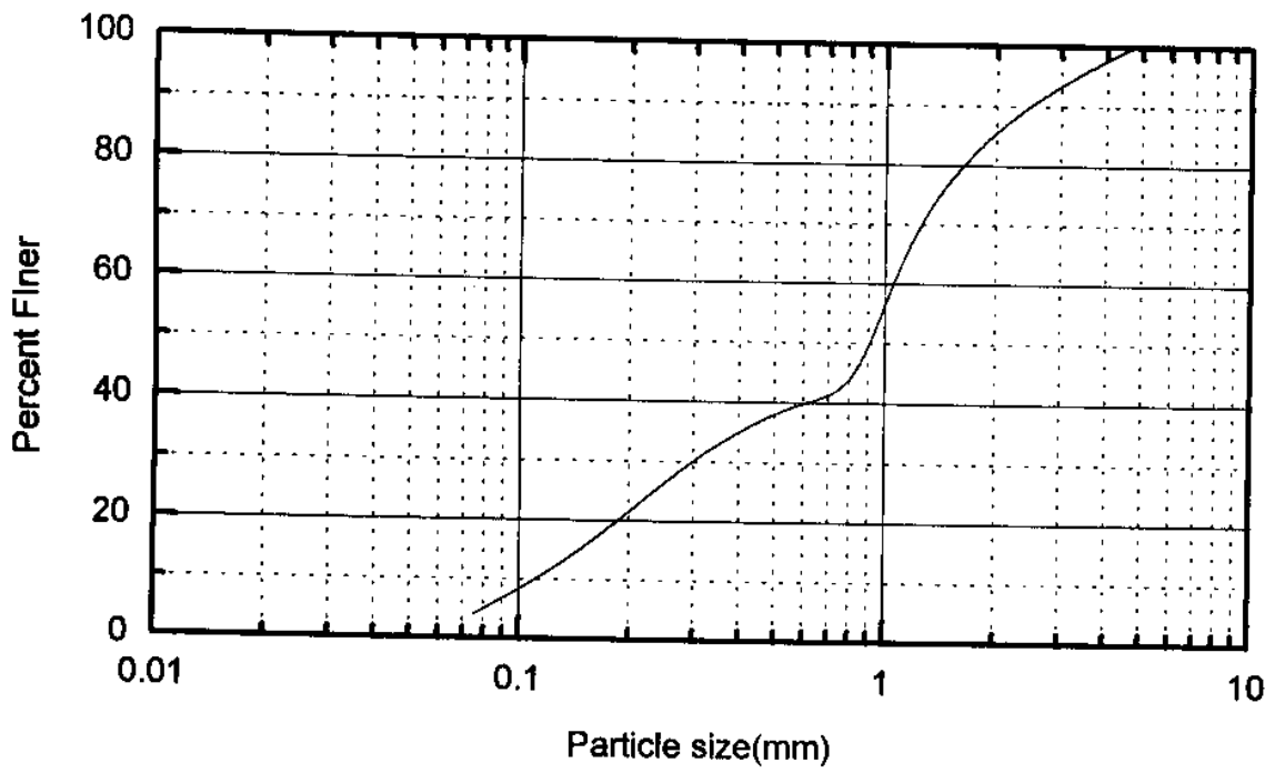
Fig 11 Grainsize distribution curve (Dharmavaram village)
