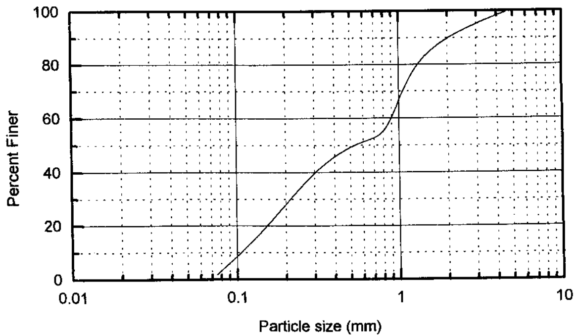
Fig 10 Grainsize distribution curve (Gokavaram village)
