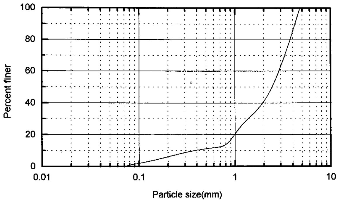
Fig 20 Grainsize distribution curve (T Rayavaram village)
