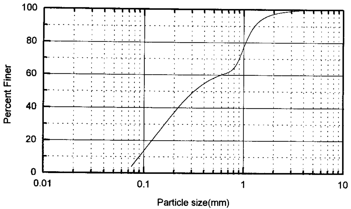
Fig 8 Grainsize distribution curve (Potuluru village)
