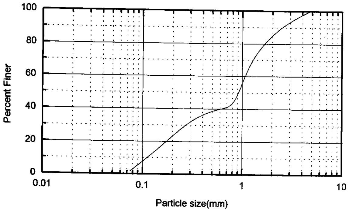
Fig 12 Grainsize distribution curve (Chebrolu village)
