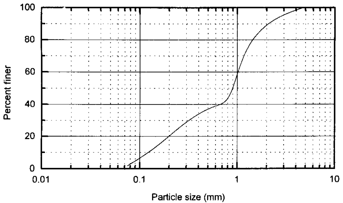
Fig 16 Grainsize distribution curve (Prathipadu village)
