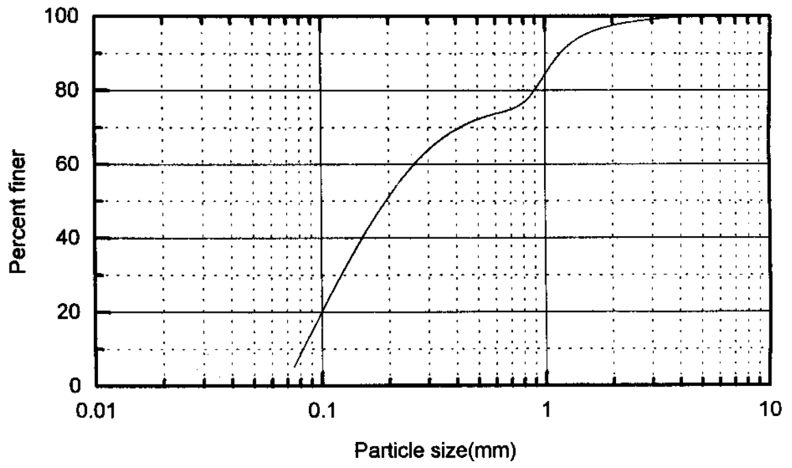
Fig 21 Grainsize distribution curve (Peddipalem village)
