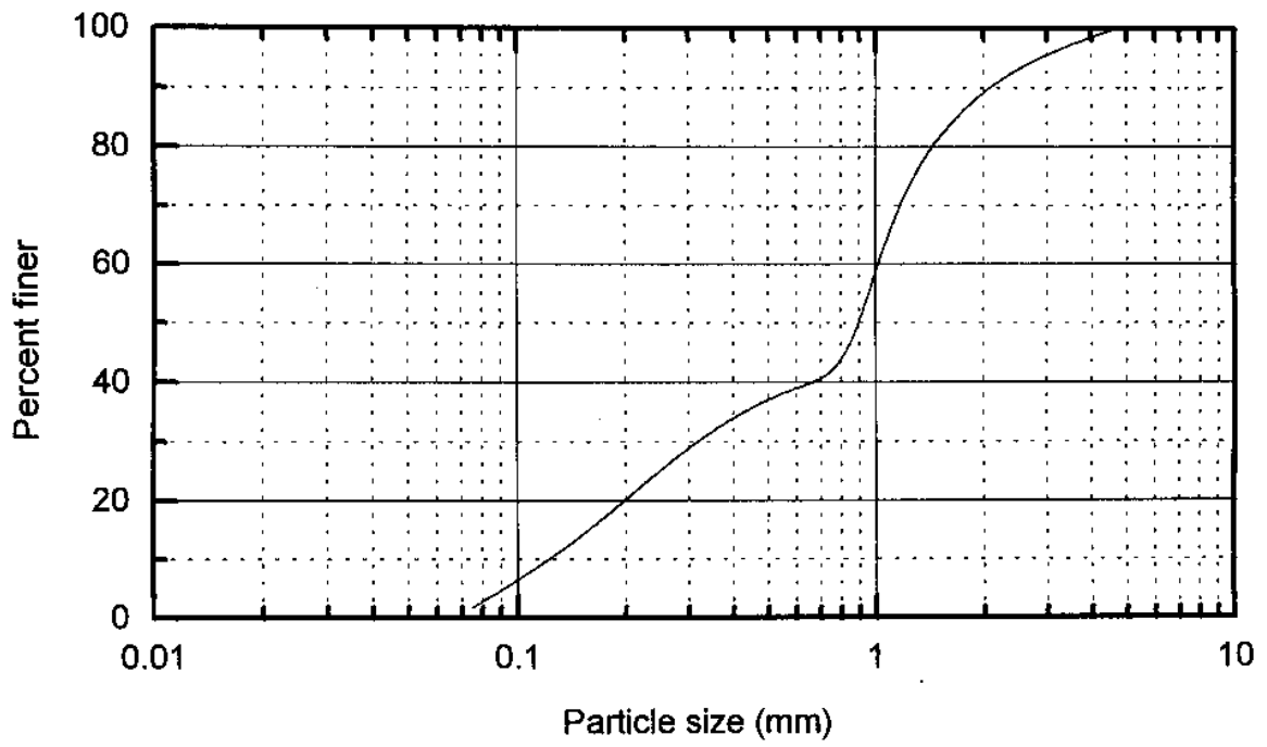
Fig 17 Grainsize distribution curve (Tatiparthi village)
