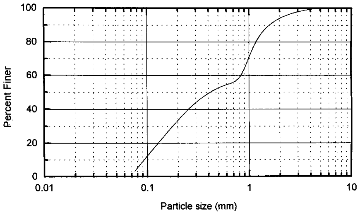
Fig 13 Grainsize distribution curve (Sarabhavaram village)
