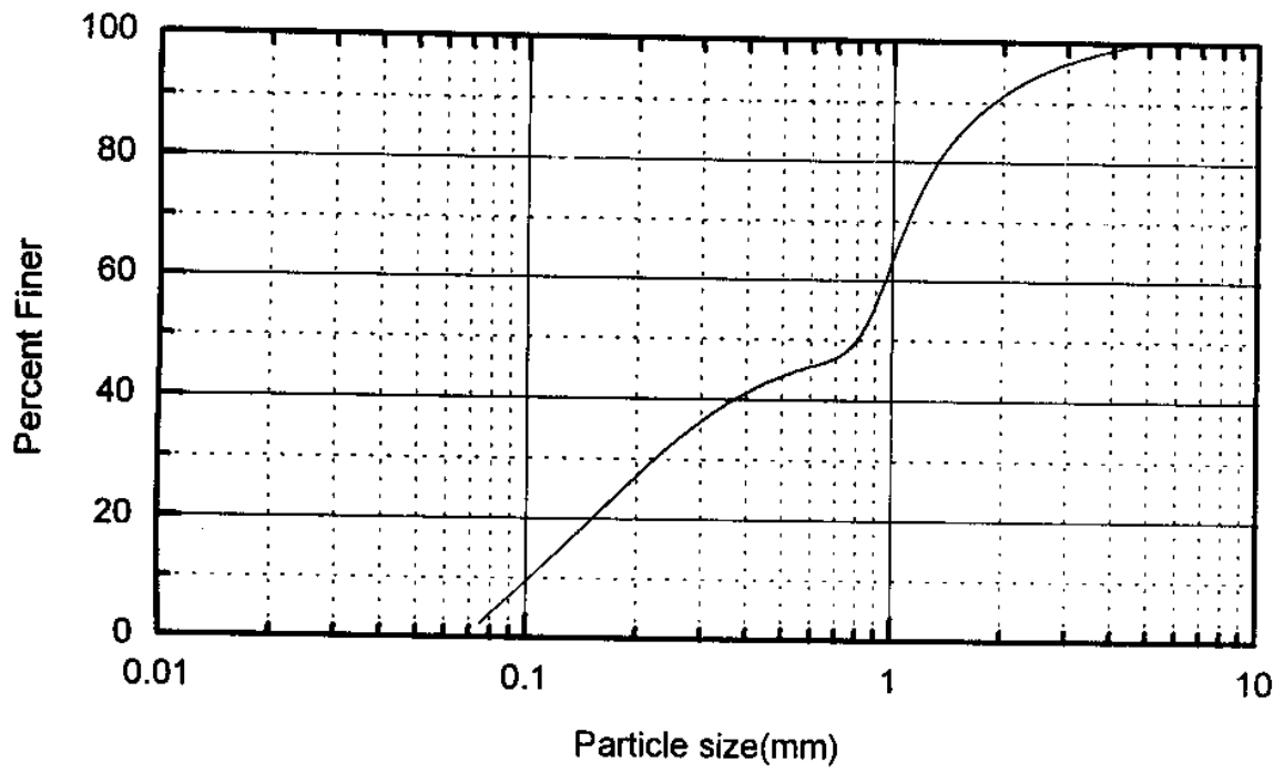
Fig 7 Grainsize distribution curve (Uttarkanchi village)
