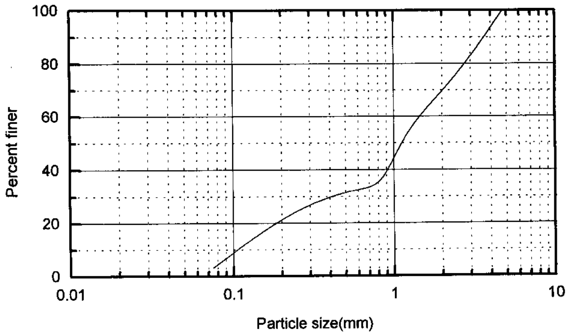
Fig 14 Grainsize distribution curve (Gollaprolu village)
