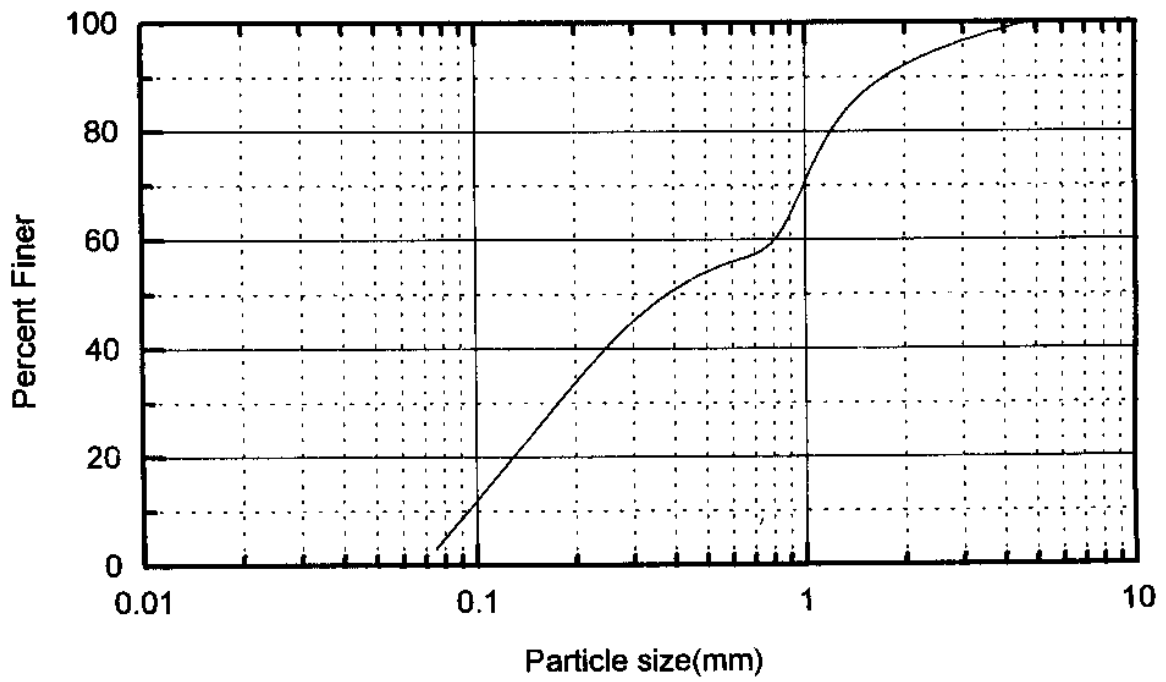
Fig 9 Grainsize distribution curve (Chintaluru village)
