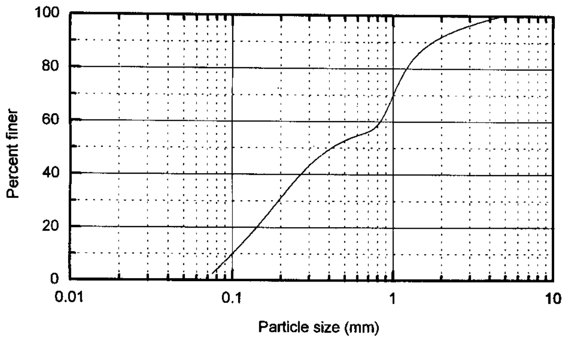
Fig 19 Grainsize distribution curve (Dontamuru village)
