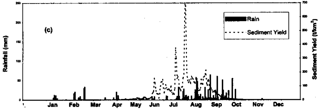
Fig. 19 Daily rainfall and suspended sediment yield at (a) Kasol (b) Suni (c) Intermittent catchment between Suni and Kasol (1994)
