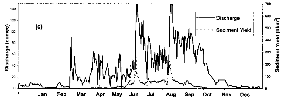
Fig. 9: Daily discharge and suspended sediment yield at (a) Kasol (b) Suni (c) Intermittent catchment between Suni and Kasol (1996)
