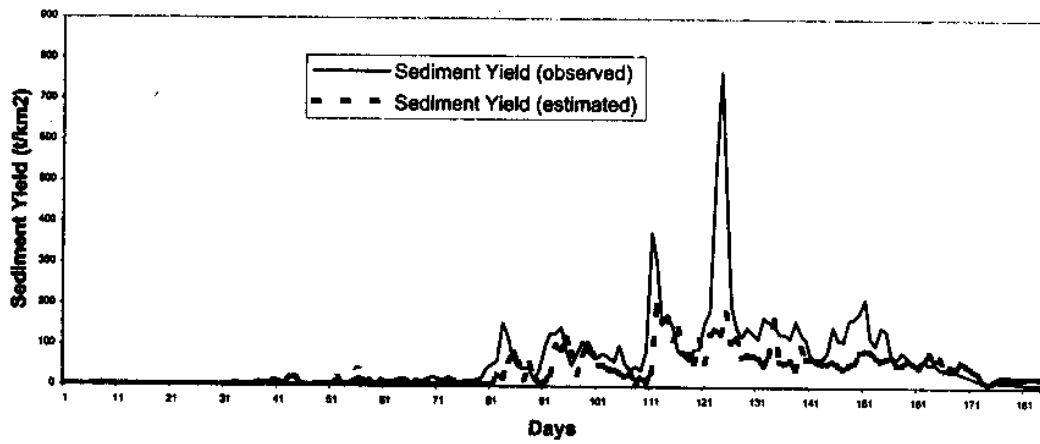
Fig.22: Daily sediment yield at (a) Kasol (b) Suni (c) Intermittent catchment (1994)
