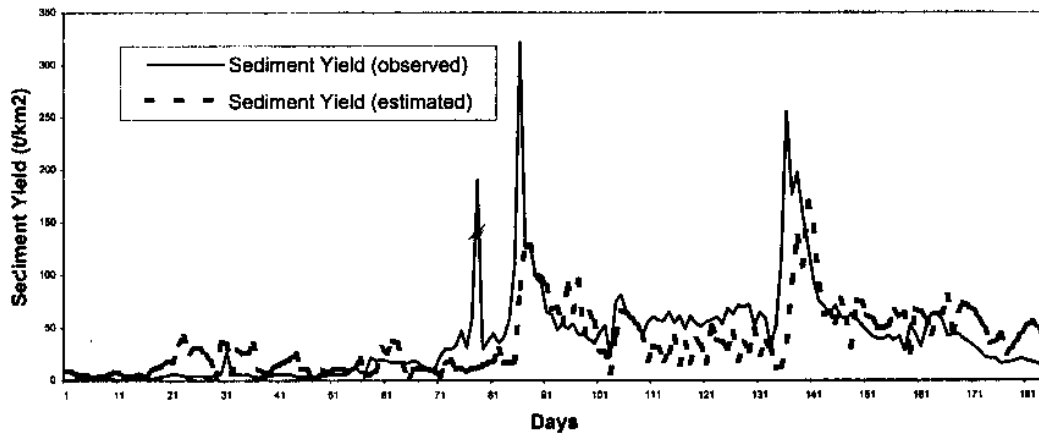
Fig 24 Daily sediment yield at (a) Kasol (b) Suni (c) Intermittent catchment (1996)
