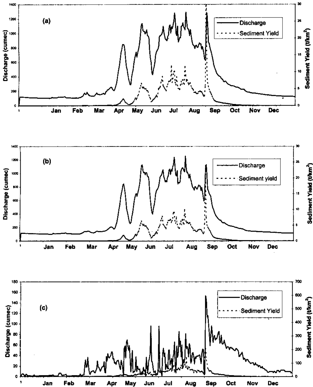
Fig. 8: Daily discharge and suspended sediment yield at (a) Kasol (b) Suni (c) Intermittent catchment between Suni and Kasol (1995)
