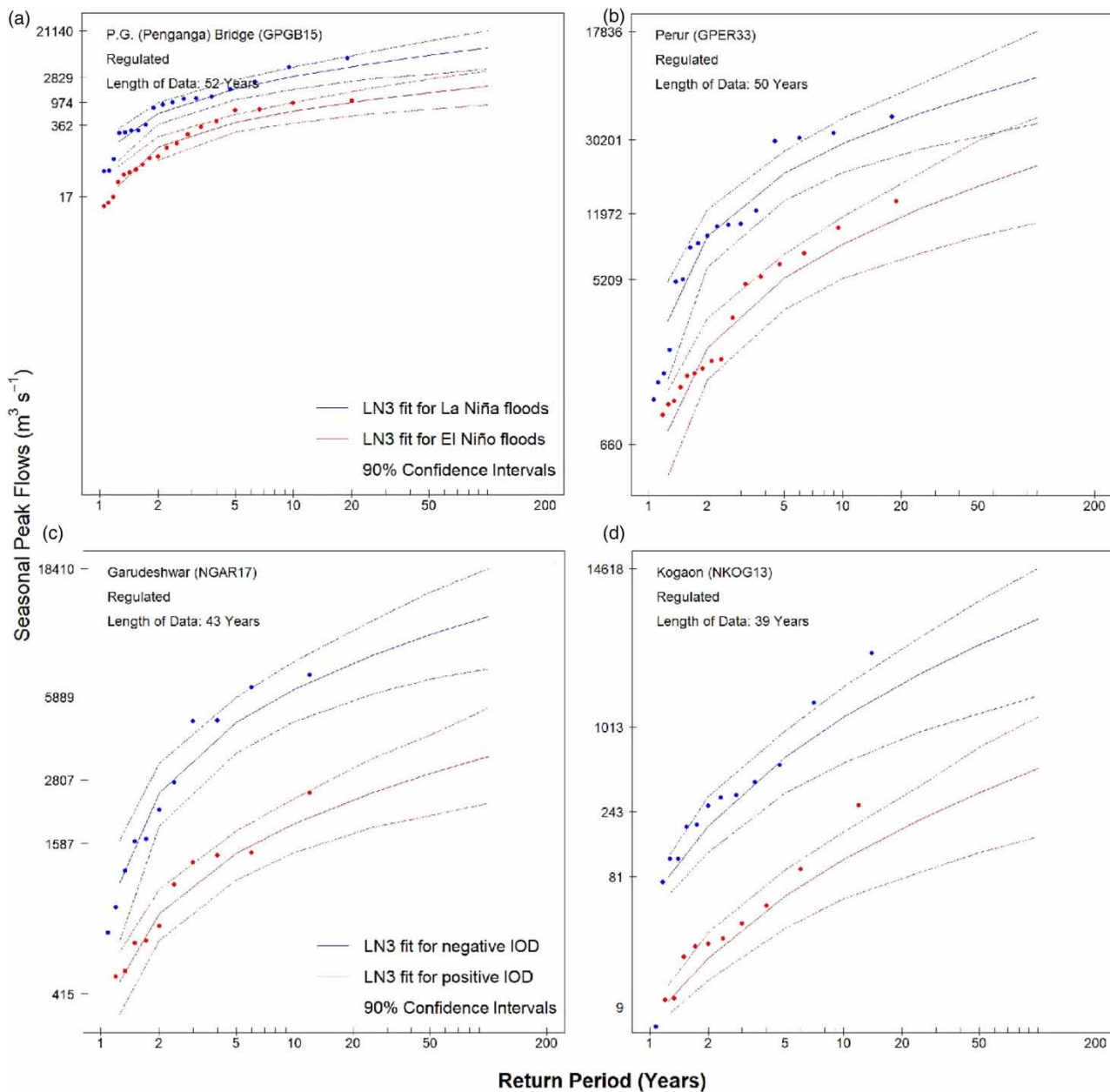
Figure 7 | 3-Parameter Lognormal (LN3) flood frequency curves (solid lines) and their 90% confidence intervals (dashed lines) for the northeast monsoon seasonal (NE) peak flows in two selected gauges from the Godavari River basin, (a) P.G. (Penganga) Bridge, (b) Perur, stratified according to El Niño ( ONI_{OND} \geq -0.5 ) and La Niña ( ONI_{OND} \leq -0.5 ) episodes of El Niño-Southern Oscillation (ENSO) pattern and in two selected gauges from the Narmada River basin, (c) Garudeshwar and (d) Kogaon, stratified according to positive ( DMI_{OND} \geq 0.1 ) and negative ( DMI_{OND} \leq -0.1 ) episodes of Indian Ocean Dipole (IOD).
