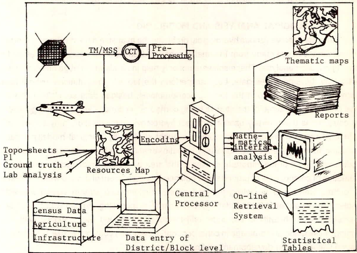
Fig. 12 : Flow Chart for Data Management System for NRDMs
