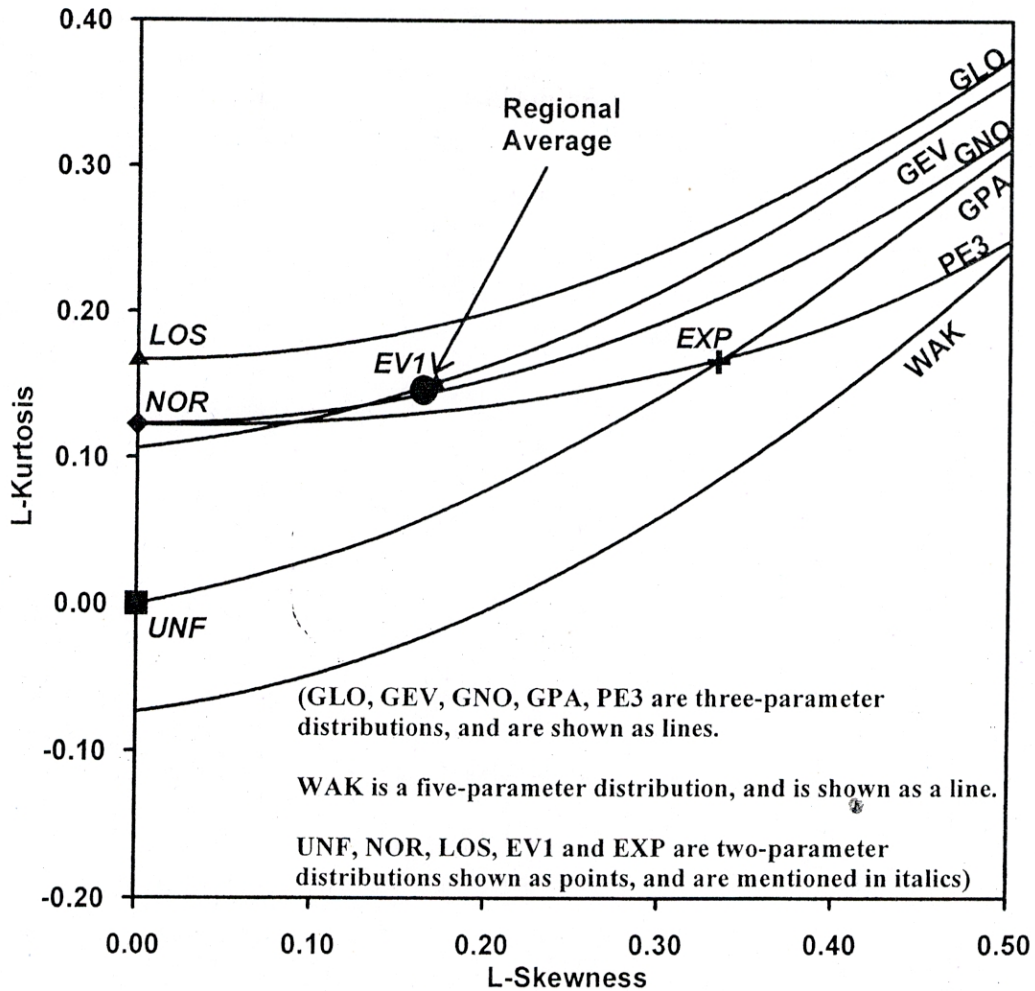
Figure 1. L-moment ratio diagram for Subzone 1(f)
