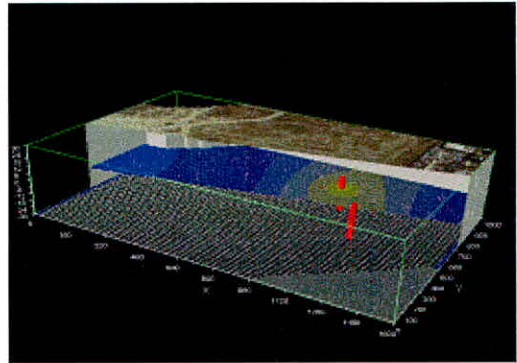
Fig. 9 Animation of a concentration plume. The source of the plume is located on the ground surface to the left of the model. Due to pumping in the lower aquifer and recharge at the ground surface, the concentration plume flows through the confining layer (not displayed) and reaches the lower aquifer.
