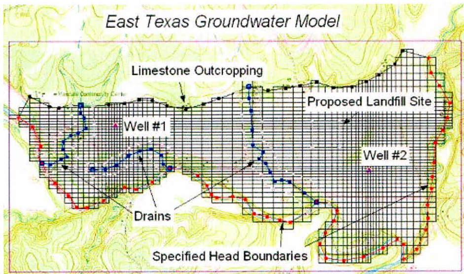
Fig. 4 Finite element grids created by GMS
