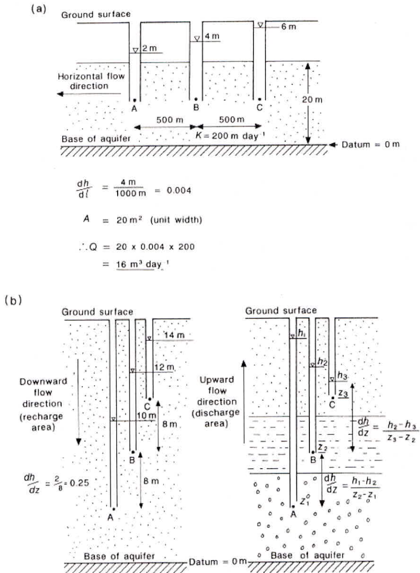
Fig. 5 Determination of groundwater flow direction and hydraulic head gradient from piezometer measurements for (a) horizontal flow and (b) vertical flow. The elevation of the water level indicating the hydraulic head at each of the points A, B and C is noted adjacent to each piezometer.
