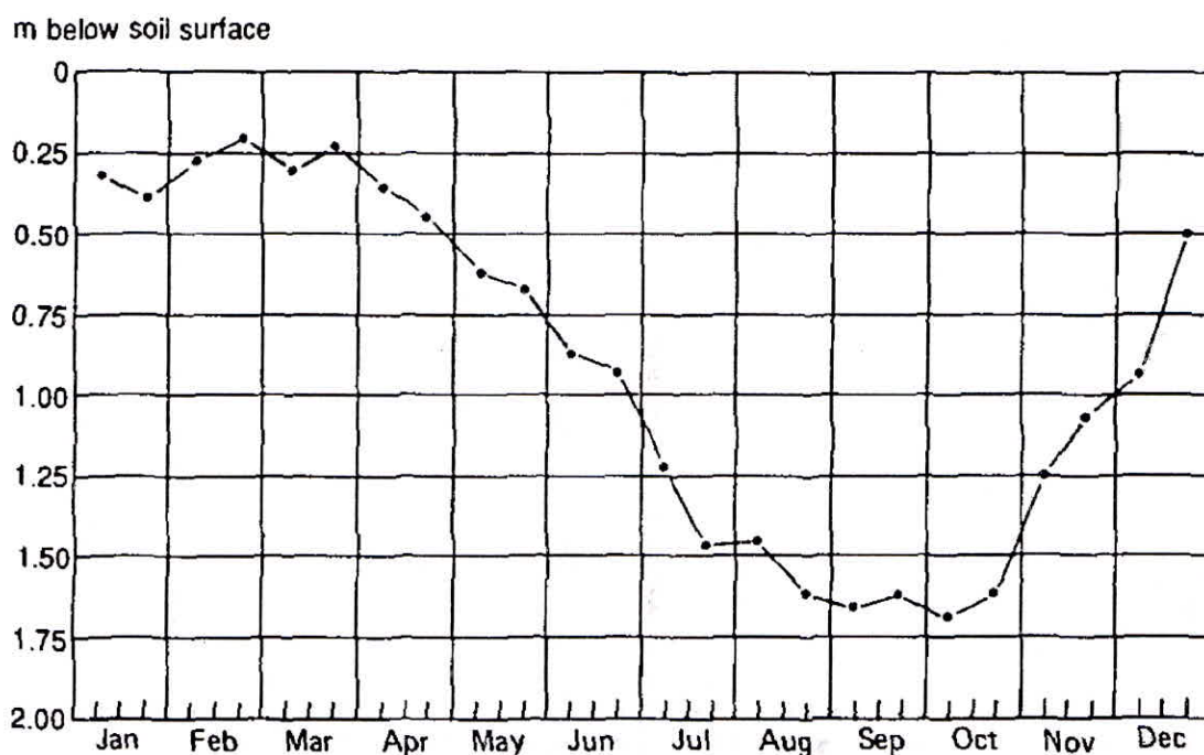
Figure 1: Hydrograph of a Water Table Observation Well
