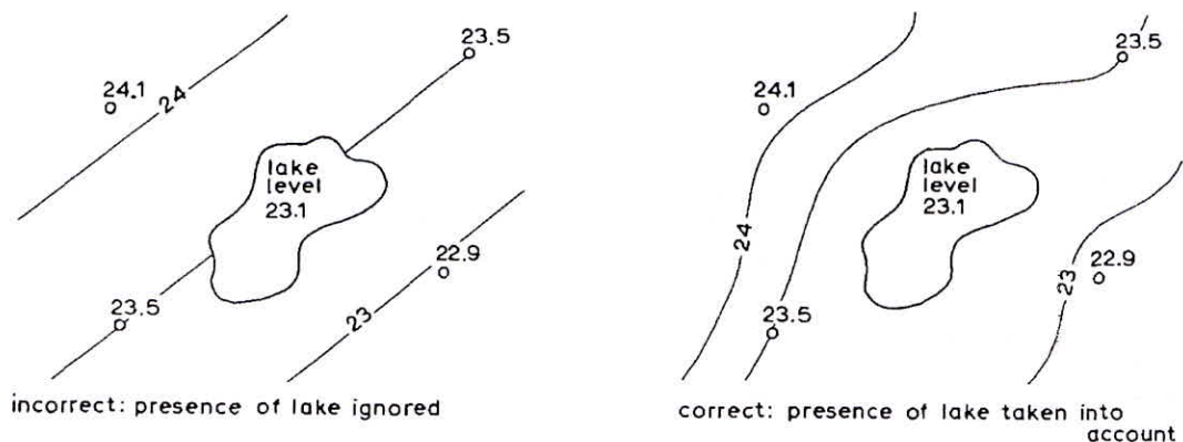
Figure 3: Example of Water Table-Contour Lines
