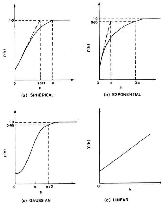
Figure 7: Theoretical Models of Variogram
