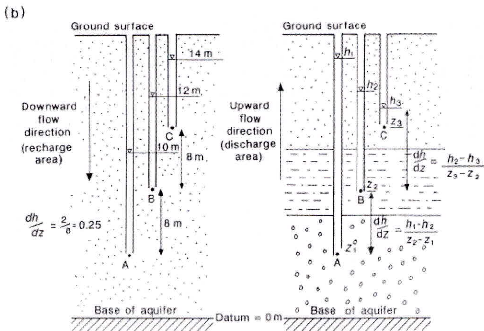
Figure 5: Determination of groundwater flow direction and hydraulic head gradient from piezometer measurements for (a) horizontal flow and (b) vertical
