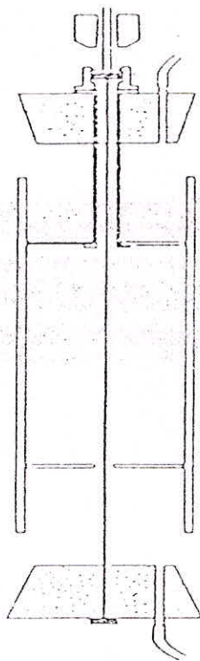
Figure 7. Kemmerer Sampler
