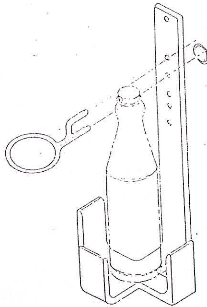
Figure 4. Sample Bottle Holder for Manual Sampling
