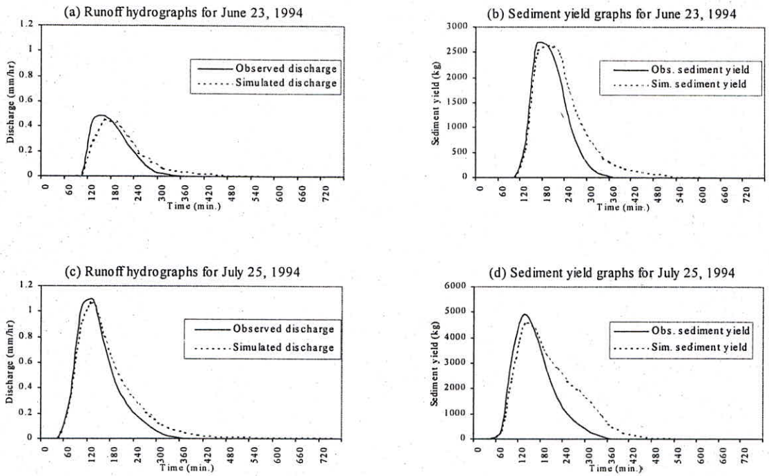
Fig. 9: Runoff hydrographs and sediment yield graphs for validation events
