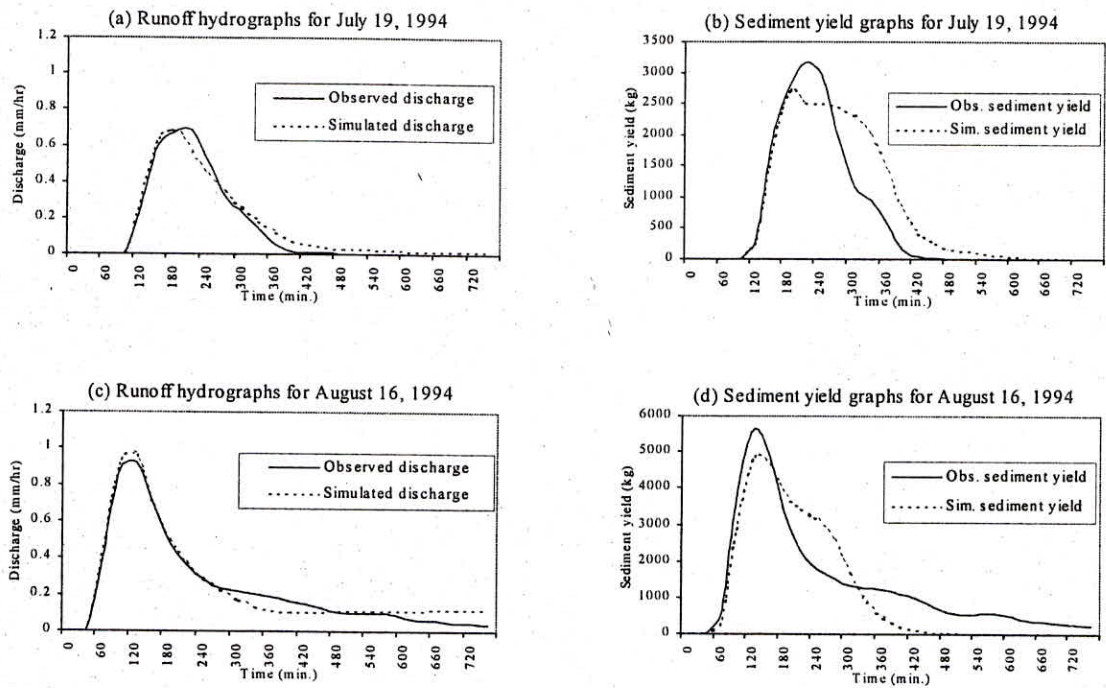
Fig. 8: Runoff hydrographs and sediment yield graphs for calibration events
