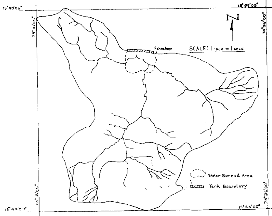
Fig. 1. Catchment Area of Rakaskop tank.
