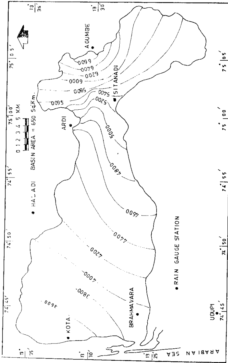
FIG. 3.1.1.2. Isohyetal Map of Sitanadi Basin
