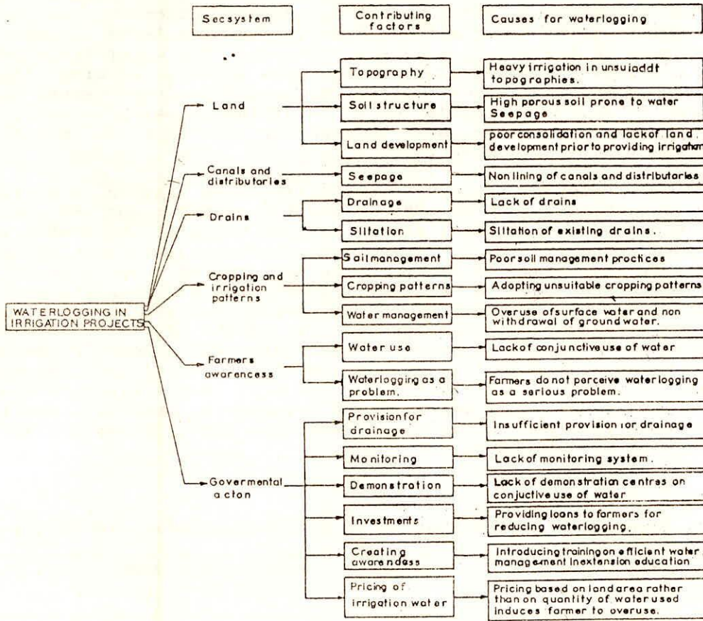
Causes of waterlogging in irrigation projects (MOWR 1991)
