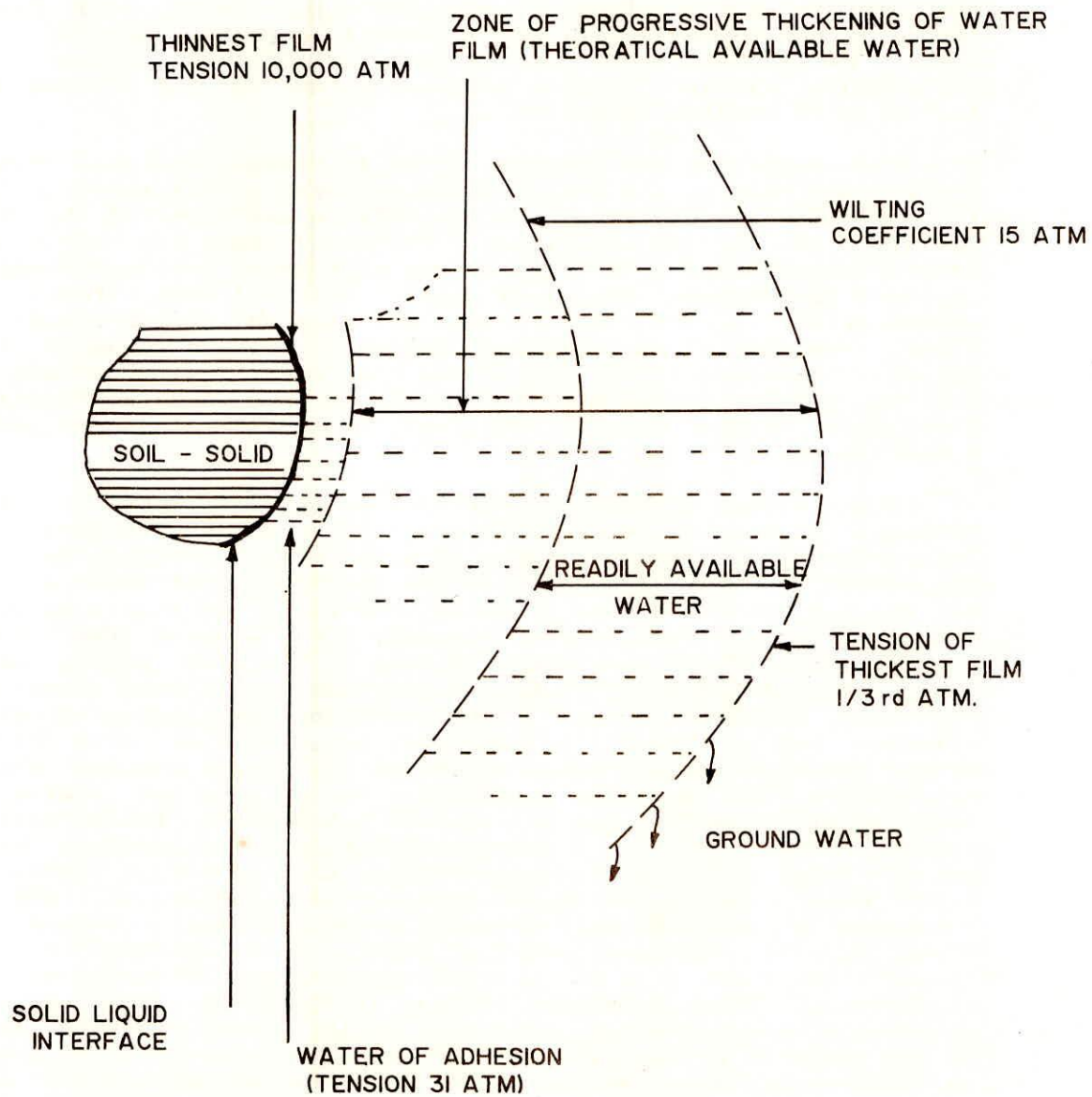
FIG.2. SOIL WATER-SHOWING PROGRESSIVE THICKENING OF WATER
